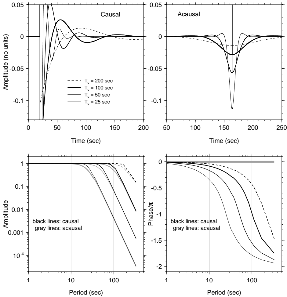
Figure 1. Results of filtering an impulse with amplitude of 256 with both causal and acausal filters, with corner periods of 200, 100, 50, and 25 sec. The time-domain responses as well as the Fourier amplitude and phase spectra are shown (the Fourier spectra were computed by taking the FFT of the time-domain spike, using program ampph4lc.for; the results agree with the theoretical results). The time series for the causal filters have been shifted to the left, compared to the location of the responses for the acausal filters, in order to capture most of the tails of the responses. Note that the time-domain impulse responses shown in the top row are plotted at a greatly expanded scale to show details; the responses are actually dominated by impulses of amplitude 256. The legend for corner periods ( T_c ) shown in the upper left plot is the same for all plots. The plots of the amplitude and phase responses combine both the causal and acausal filter responses; the acausal responses are plotted using gray lines. The phase spectra have been corrected for the linear phase due to placing the impulse at a time not equal to 0.0, and the corrected phase spectra have been normalized by dividing by \pi . Note the large phase shifts for the causal filters, even for periods away from the corner periods, and the difference in the phase shifts for the different filters. In contrast, the phase shifts for the acausal filters are zero. (From Boore and Akkar, 2003.)
