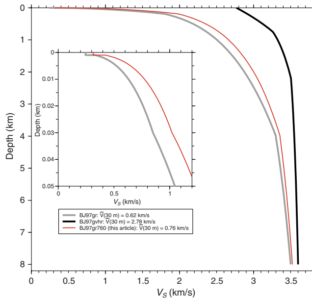
Figure 2. V_s as a function of depth for the Boore and Joyner (1997) ; BJ97 generic rock (BJ97gr) and generic very hard rock (BJ97gvhr) models, and the interpolation of those two models such that \bar{V}_s(30 \text{ m}) = 0.76 \text{ km/s} (BJ97gr760). The color version of this figure is available only in the electronic edition.
