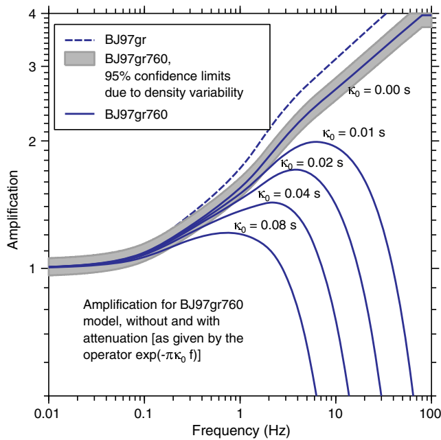
Figure 3. The combined effect of the amplification for the BJ97gr760 model in Table 1 and the attenuation given by \exp(-\pi\kappa_0 f) . The shaded band around the \kappa_0 = 0.0 s curve indicates the 95% confidence limits due to the uncertainty in the density–velocity relation (see text). For comparison, the dashed line is the amplification for the BJ97gr velocity model, using the densities computed using the procedure in this article. This figure is equivalent to figure 8 in Boore and Joyner (1997). The color version of this figure is available only in the electronic edition.
