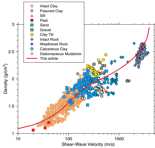
Figure 1. The relation between density and shear-wave velocity ( V_s ) proposed in this article, compared with data from Mayne (2001) ; also in Mayne et al., 2002 ). More data than shown here were used to establish the curve for larger velocities; see Gardner et al. (1974) and Brocher (2005) . The color version of this figure is available only in the electronic edition.
