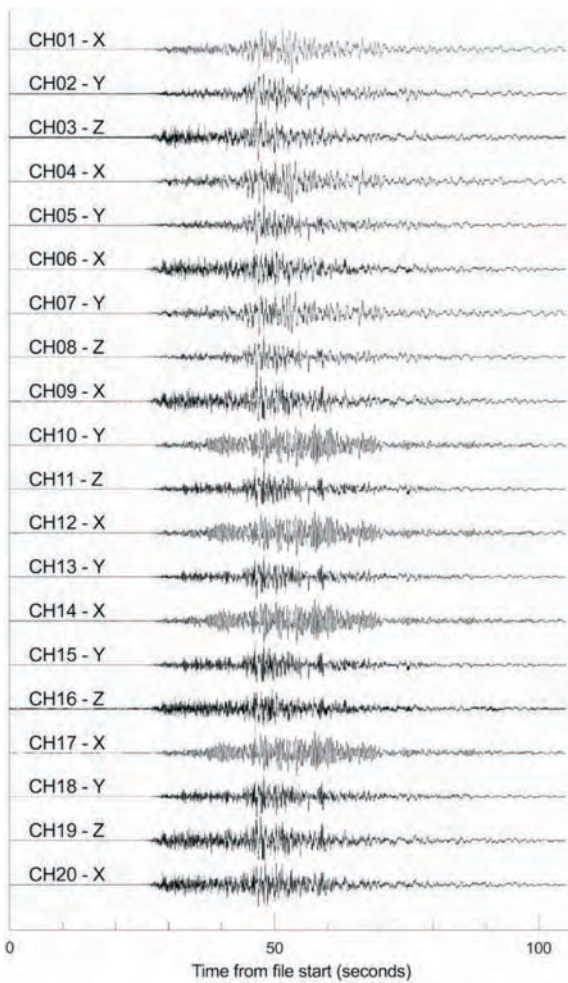
Fig. 17. Waveforms recorded by the strong-motion array (TTNBA0) at the National Taitung Senior High Commercial and Vocational School from the first Pingtung earthquake. The channel number corresponds to the accelerometer number shown in Fig. 16. Please note that the waveform amplitudes are not shown in true scale (they are normalized to fit within the plotting space).
