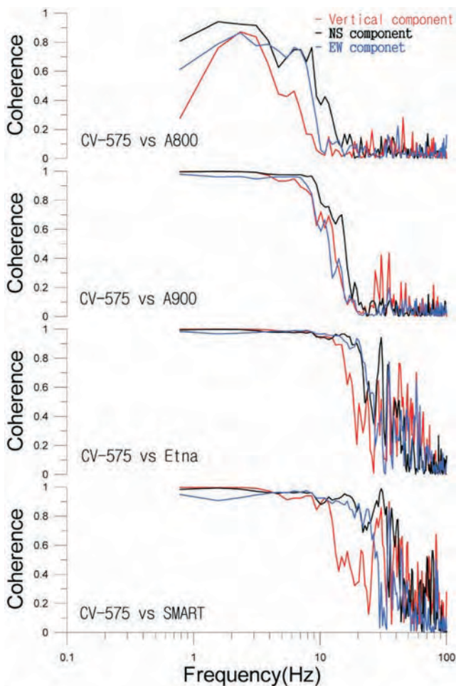
Fig. 8. Waveform coherence at Station TAP117 between the record of the second Pingtung earthquake from the CV-575 accelerograph and the records from the A800, A900, Etna, and SMART-24A accelerographs.
