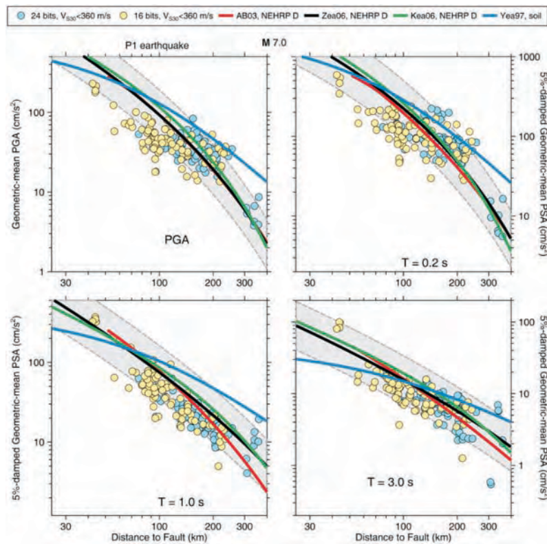
Fig. 13. Comparison of earthquake P1 data for 16- and 24-bit instruments and ground-motion predictions for indicated references (AB03 = Atkinson and Boore 2003; Kea06 = Kanno et al. 2006; Yea97 = Youngs et al. 1997; Zea06 = Zhao et al. 2006). The curves are plotted for a “soft soil” site class (NEHRP D). The gray bands show the plus and minus one standard deviations for the Zea06 GMPEs.
