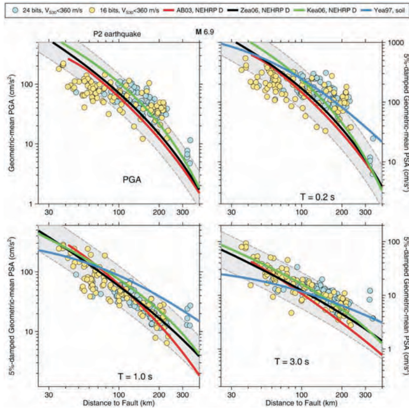
Fig. 15. Comparison of earthquake P2 data for 16- and 24-bit instruments and ground-motion predictions for indicated references (AB03 = Atkinson and Boore 2003; Kea06 = Kanno et al. 2006; Yea97 = Youngs et al. 1997; Zea06 = Zhao et al. 2006). The curves are plotted for a “soft soil” site class (NEHRP D). The gray bands show the plus and minus one standard deviations for the Zea06 GMPEs.
