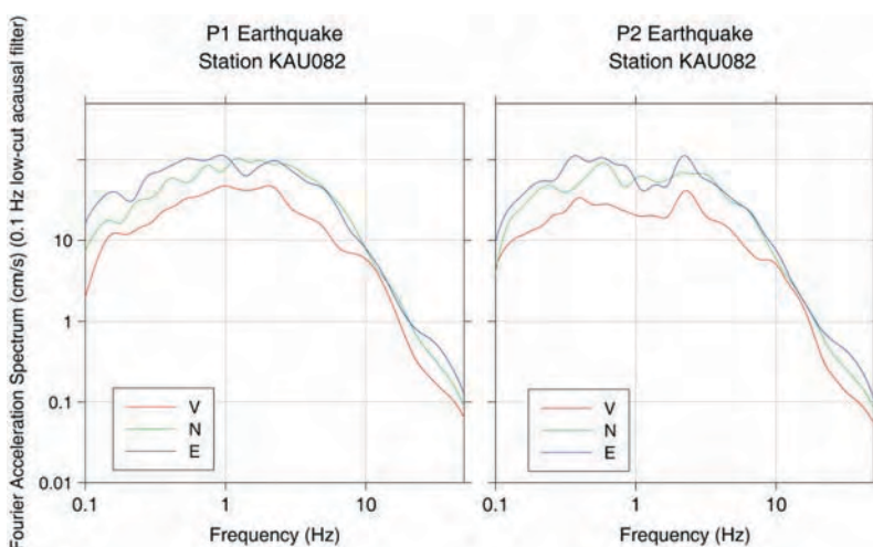
Fig. 7. Fourier acceleration spectra for both events at station KAU082, one of the closest stations. To make it easier to compare the spectra, they have been smoothed over log-spaced frequencies, with a Konno and Ohmachi (1998) smoothing operator with a width of 0.4 of a decade.
