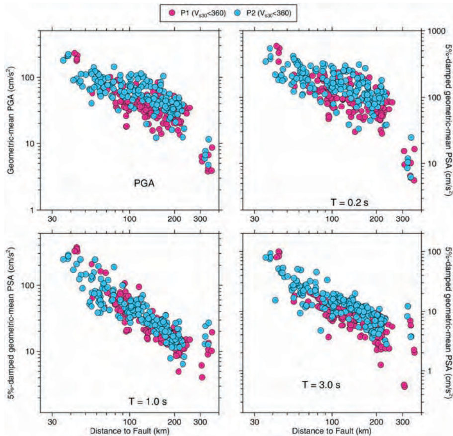
Fig. 11. Comparison of ground motions for the two events for “soil” sites. Shown are the geometric means of the two horizontal components.
