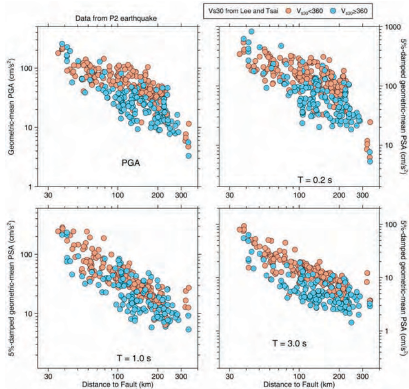
Fig. 10. Ground-motions vs. distance for the second earthquake (P2), separated by Vs30 values at each station. Shown are the geometric means of the two horizontal components.
