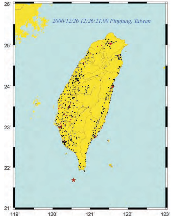
Fig. 1. Map showing the locations of the triggered stations from the first Pingtung earthquake. Free-field accelerograph stations are plotted as small black "diamonds", and strong-motion arrays in buildings or bridges are plotted as red "dots". The earthquake epicenter is shown as "star".
