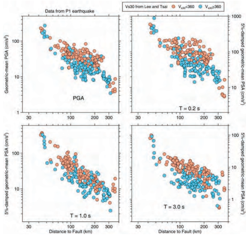
Fig. 9. Ground-motions vs. distance for the first earthquake (P1), separated by Vs30 values at each station. Shown are the geometric means of the two horizontal components.
