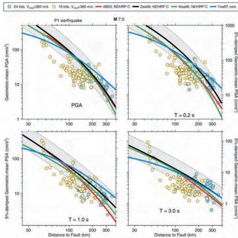
Fig. 12. Comparison of earthquake P1 data for 16- and 24-bit instruments and ground-motion predictions for indicated references (AB03 = Atkinson and Boore 2003; Kea06 = Kanno et al. 2006; Yea97 = Youngs et al. 1997; Zea06 = Zhao et al. 2006). The curves are plotted for a “stiff soil” site class (NEHRP C). The gray bands show the plus and minus one standard deviations for the Zea06 GMPEs.
