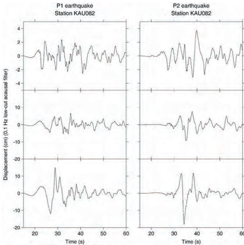
Fig. 6. Displacement time series for both events at station KAU082, one of the closest stations.
