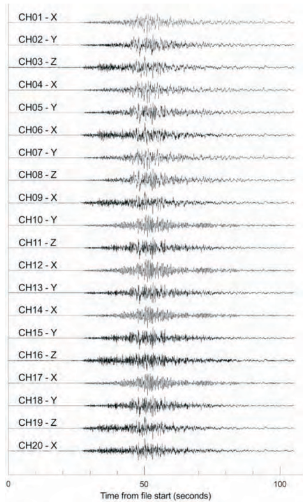
Fig. 18. Waveforms recorded by the strong-motion array (TTNBA0) at the National Taitung Senior High Commercial and Vocational School from the second Pingtung earthquake. The channel number corresponds to the accelerometer number shown in Fig. 16. Please note that the waveform amplitudes are not shown in true scale (they are normalized to fit within the plotting space).
