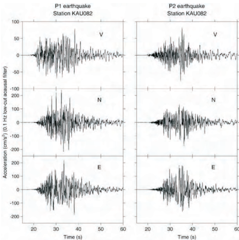
Fig. 4. Acceleration time series for both events at station KAU082, one of the closest stations.
